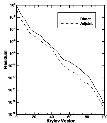
Fig. 2 Convergence rates for direct and adjoint modes.
