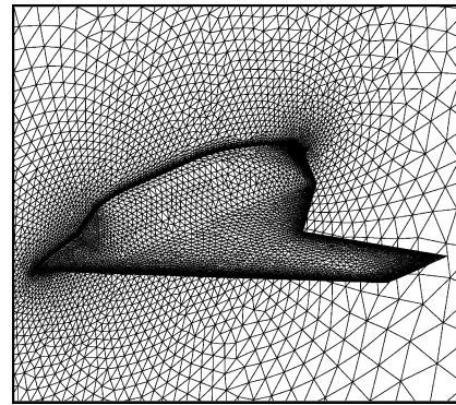
Fig. 5 Surface grid for morphing aircraft in cruise configuration.
