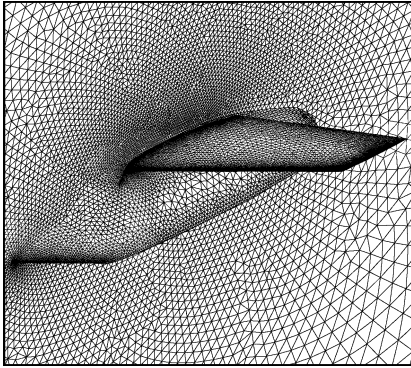
Fig. 3 Surface grid for morphing aircraft in dash configuration.
