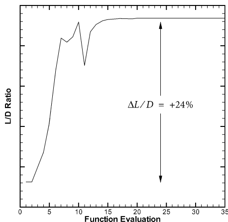
Fig. 6 Lift-to-drag ratio during unconstrained optimization of cruise configuration.
