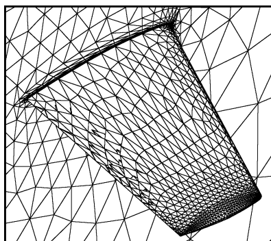
Fig. 1 ONERA M6 grid used for evaluating linearizations.
