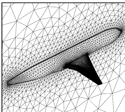
Fig. 7 Surface grid for slotted wing-body configuration.
