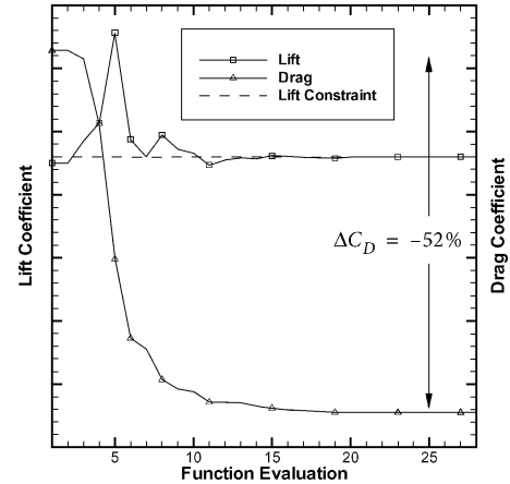
Fig. 4 Lift and drag coefficients during constrained optimization of dash configuration.
