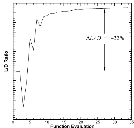
Fig. 8 Lift-to-drag ratio during unconstrained optimization of wing-body configuration.
